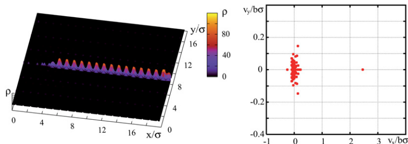
Fig. 6. Triangular Morse lattice. Cumulative picture of the peaks of atom core electron density illustrating long lasting and hence highly stable soliton-like excitations running along a crystallographic axis in a 2d triangular Morse lattice (“bubble chamber representation”). The right picture shows the velocity distribution of the lattice units. The peak in the x -direction corresponds to the propagating soliton, the lateral distribution in y -direction corresponds to oscillations transverse to the direction of the soliton propagation. Parameter values: N = 400 , b\sigma = 4 , \lambda = 0.3 and T = 0.01 .
