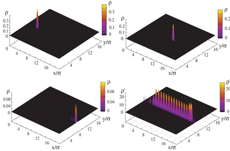
Fig. 5. Triangular Morse lattice with atoms as units. Density of atom core electrons after retaining only the highest peaks. The sequence of three snapshots, corresponding to three time instants, illustrates the long lasting quasi-1d solitonic excitations running along a crystallographic axis. The initial condition is an “optimized” Toda profile as explained in the main text. The last figure is a “bubble-chamber-representation” (including memory), i.e., a cumulative plot of many consecutive snapshots for the given time interval at the prescribed final time instant. Parameter values: N = 400 , b\sigma = 4 , \lambda = 0.3 and T = 0.01 .
