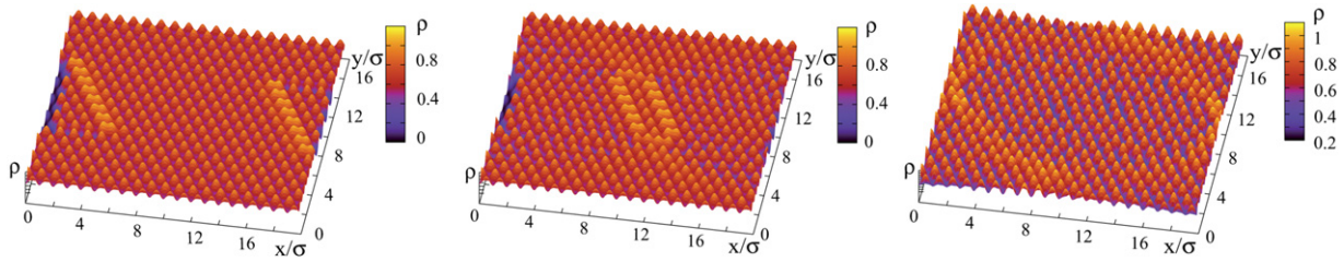
Fig. 2. Triangular Morse lattice. Head-on collision of two oppositely moving solitons: t = 0 (initial configuration; left panel), t = 4 (near collision; center panel) and t = 8 (after collision; right panel). All dots correspond to peaks in Gaussian atom core electron densities as indicated in the main text. We see the enhanced overlapping of the densities which is a signature of the underlying local mechanical lattice compressions. Parameter values: N = 400 , b\sigma = 4 , \lambda = 0.3 , \gamma_0 = 10^{-5} and T = 0.01 (note that this temperature corresponds to quite a “cold” lattice hence to a practically purely mechanical problem).
