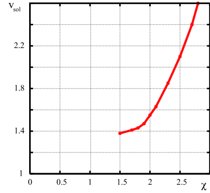
Fig. 1. Triangular Morse lattice. N = 400 ( 20 \times 20 ) atoms or lattice sites. Velocity of soliton-like excitations in units of the 1d (linear) sound velocity represented as a function of the soliton (reciprocal) width.
