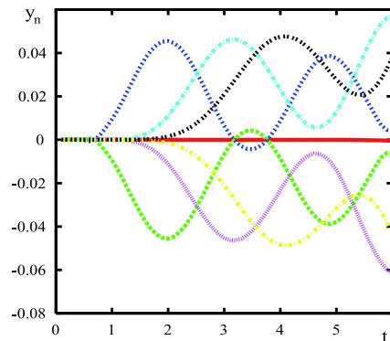
Fig. 4. Triangular Morse lattice. Time evolution in the atomic rows adjacent to the (central) one in which a high energy soliton-like excitation is running (red: soliton row; dark blue and green: nearest row; light blue and pink: next-nearest row, etc.). The (dimensionless) period of oscillations is below 3. (For interpretation of the references to colour in this figure legend, the reader is referred to the web version of this article.)
