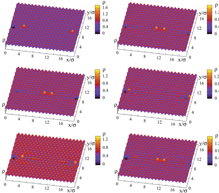
Fig. 3. Triangular Morse lattice. Head-on collision of two initially and subsequently unaltered highly-energetic nonlinear soliton-like excitations moving in opposite directions with supersonic speed at six consecutive time instants: t = 2, 3, 4, 5, 6, 7 in left-to-right, top-to-bottom zig-zag reading. Note that the solitons cross several times the boundaries, with weak transverse size. Parameter values: N = 400 , b\sigma = 4 , \lambda = 0.3 , \gamma_0 = 10^{-5} and T = 0.01 .
